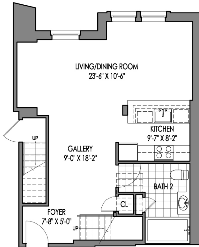
LOWER LEVEL, FIRST FLOOR: 698 SQ FEET.
